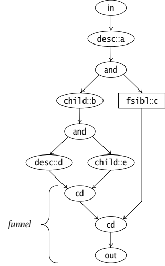
Figure 2: Transducer network for FSXP query /desc::a[child::b[desc::d]/child::e]/fsibl::c
