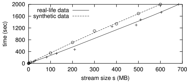
Figure 3: Varying stream size s ( q = 10 , d \leq 32 )
