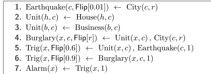
■ Figure 4 Burglar program from Figure 2 modified to use syntactic sugar
