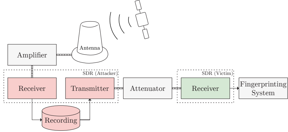
Fig. 20. Hardware setup for the replay attacks. Raw samples are captured using an SDR, then replayed directly into the fingerprinting system’s SDR over a cable.
